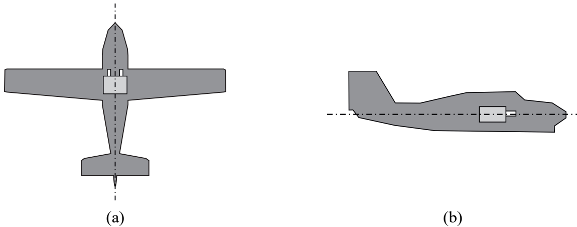
Fig. 2. Aeolus-Sense should be mounted parallel to the main axes of the airplane.
